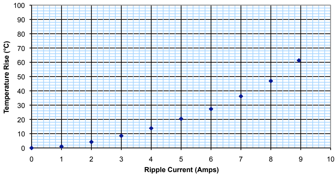
THQ5125452 Temp Rise (free air) vs. 200Hz Ripple Current
